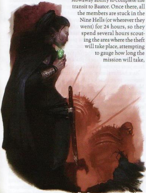
Hellbreaker
