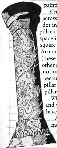
Pillar (stalagmite) or the ceiling (stalactite). Stalagmites
