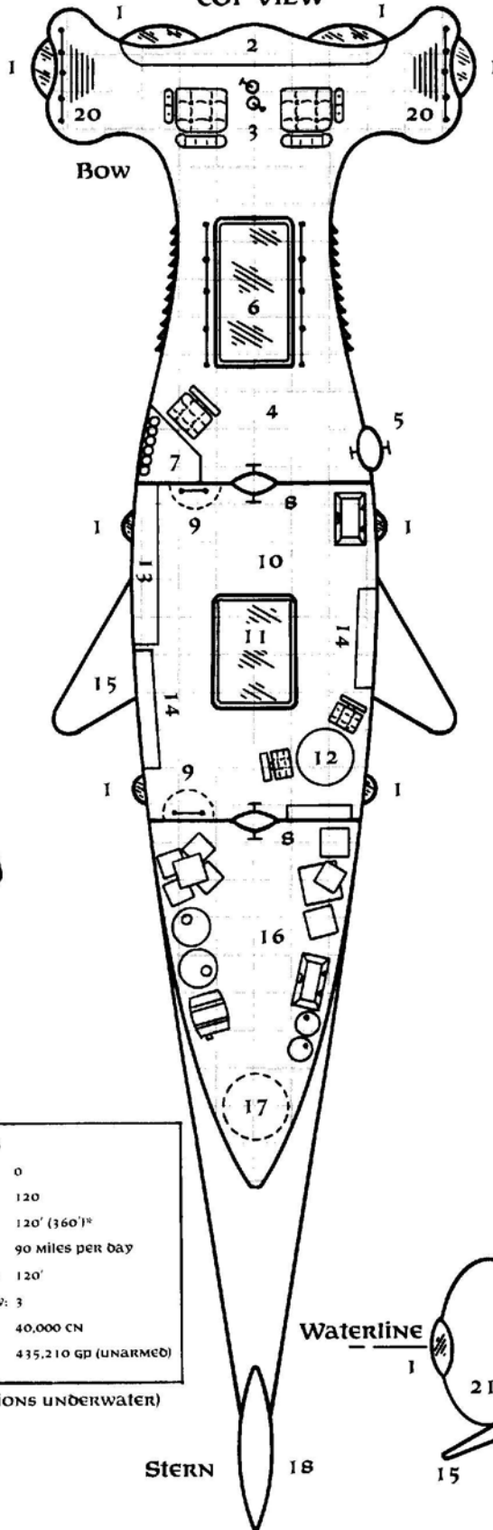
TOP VIEW
