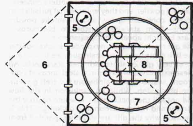
Tower gundeck level
