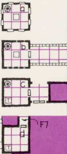
PLAN OF TOWER IN GATEHOUSES
