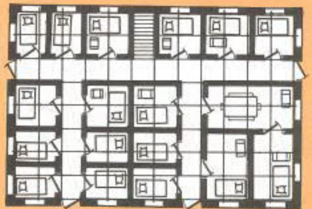
Barracks (Main Floor) Bldg. 7
