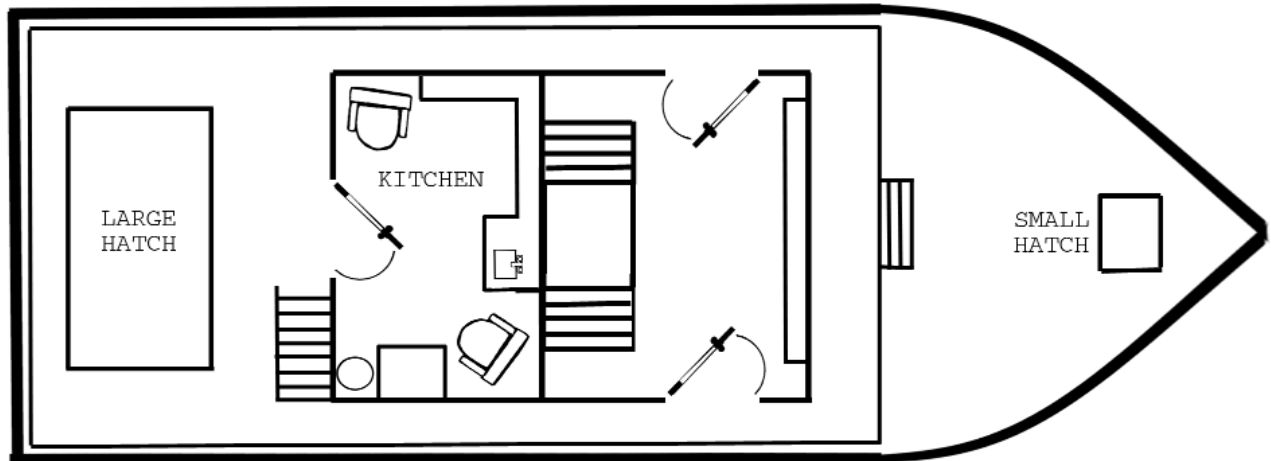
FIRST DECK
